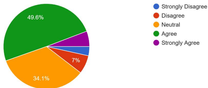
Computer Science
