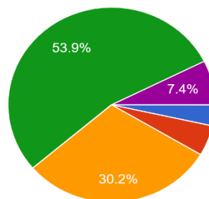
Computer Science
