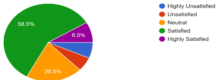
Computer Science
