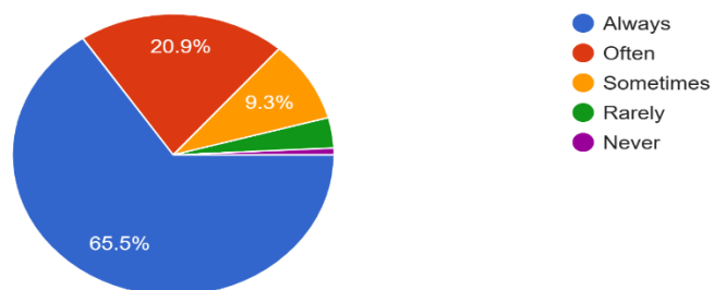
Computer Science
