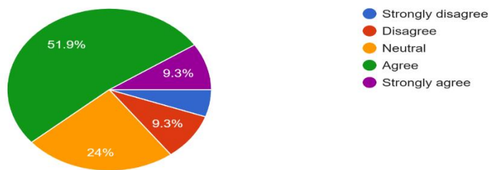
Computer Science
