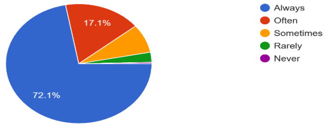
Computer Science
