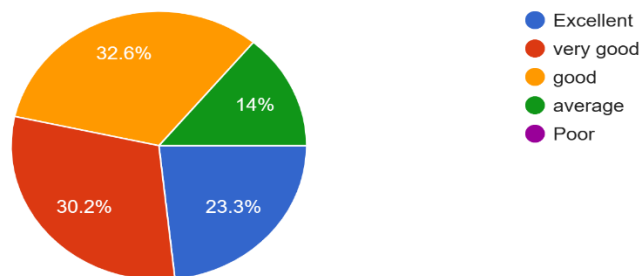
Computer Science
