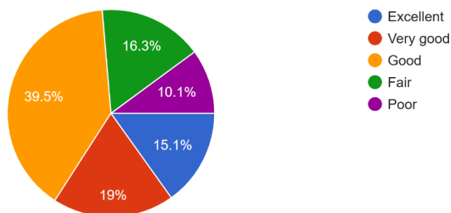
Computer Science
