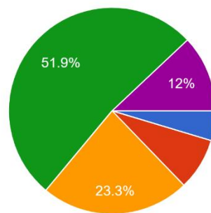
Computer Science
