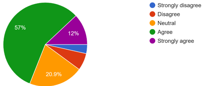
Computer Science
