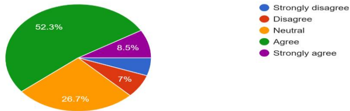
Computer Science
