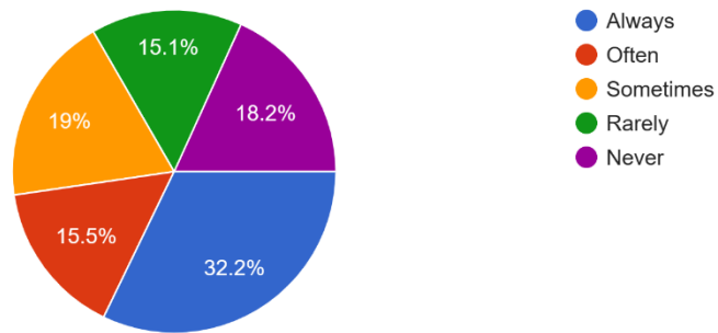
Computer Science
