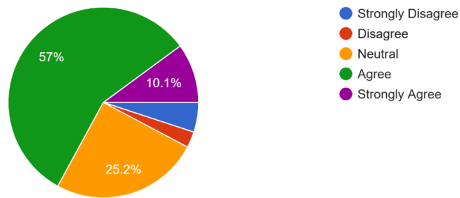
Computer Science
